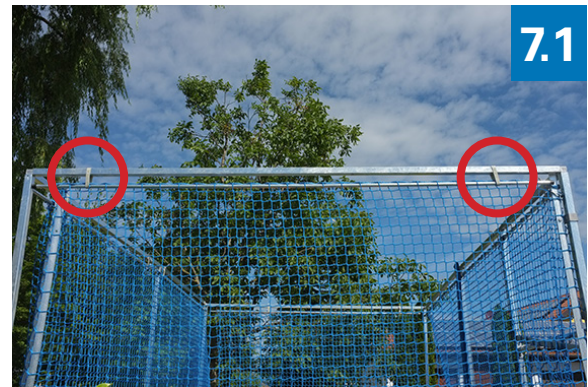
7.1- Insert round fence tube at the net attaching the net at the top fence frame by the help of the round fence tubes ( e-Round fence tube ) with straps.
